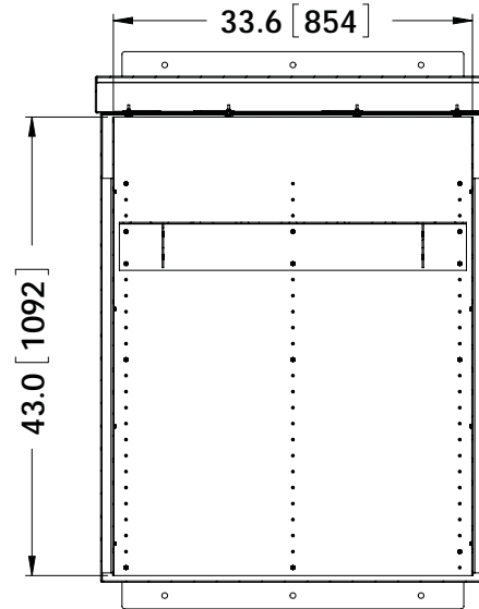
SECTION B-B (BACK PANEL)
