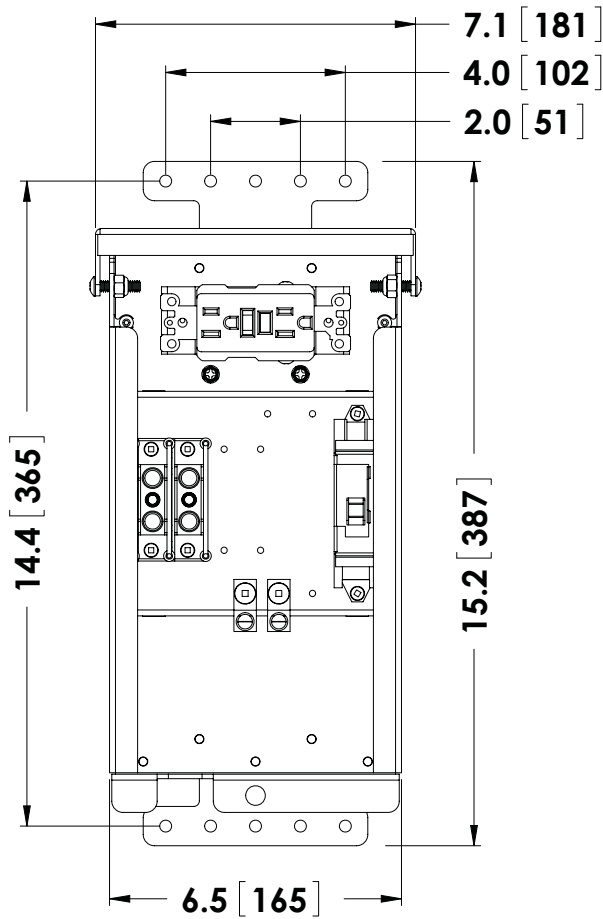
FRONT VIEW (COVER UP) (INTERIOR COVER REMOVED)
