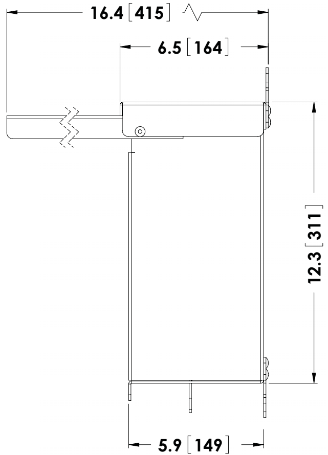
SIDE VIEW (COVER UP)
