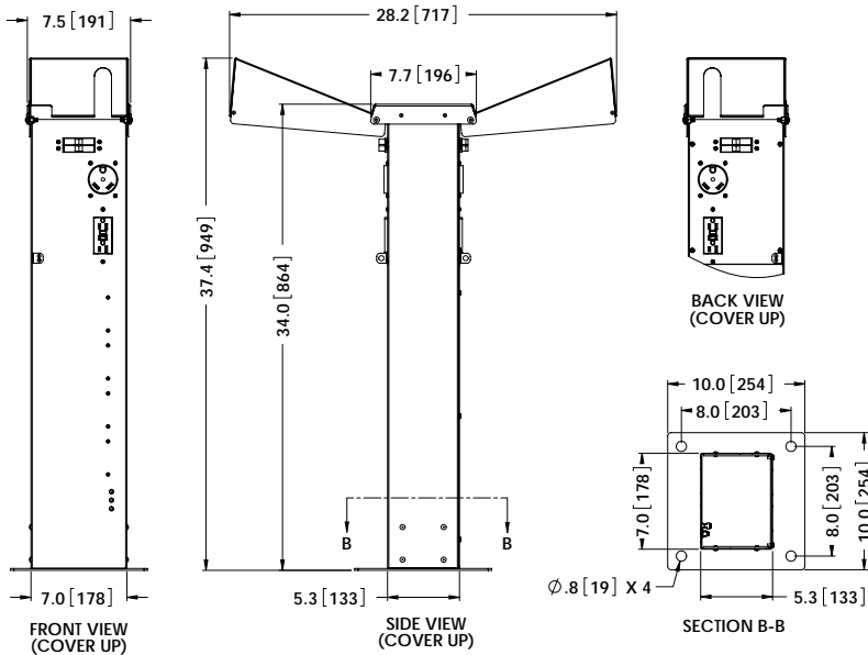
TYPICAL RVPD3 CONFIGURATION
