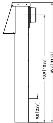
5.3 [133] 9.0 [229] 40.9 [1038] 45.6 [1158] SIDE VIEW
