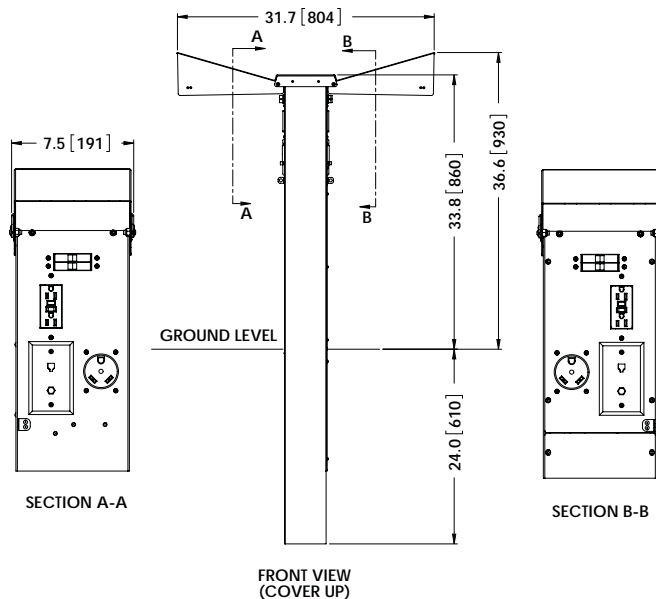
TYPICAL RVBD3-CV CONFIGURATION
