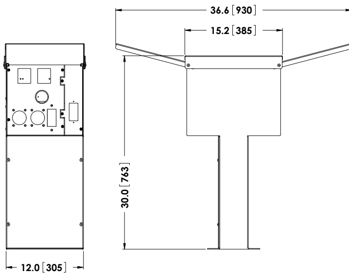
TYPICAL PRVD CONFIGURATION
