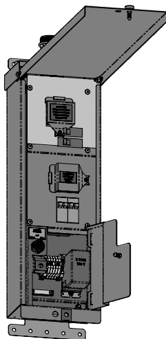
LCPSS-03 TRAFFIC/STREETLIGHT COMBINSTION PANEL 240V
