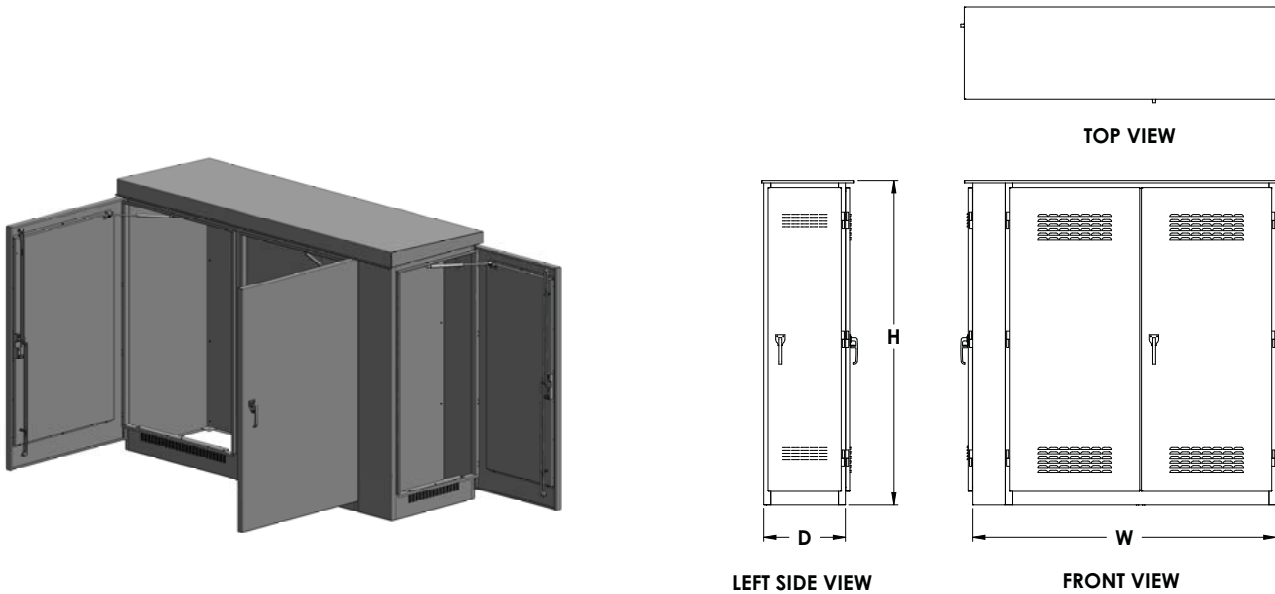
TYPICAL KXX PADMOUNT ENCLOSURE DRAWING
