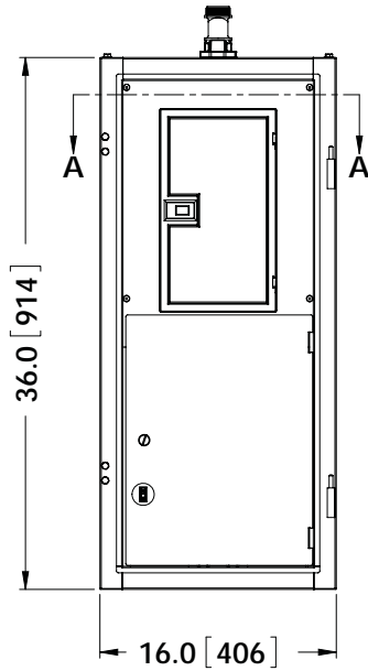
FRONT VIEW (DOOR REMOVED)
