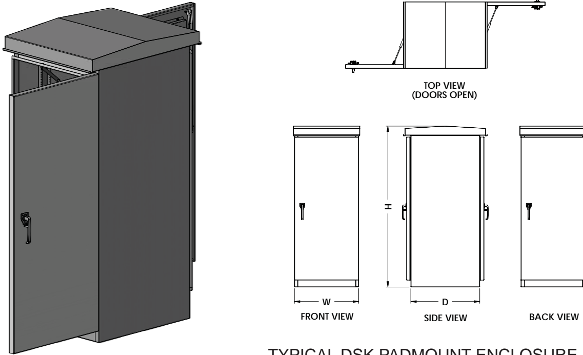
TYPICAL DSK PADMOUNT ENCLOSURE DRAWING
