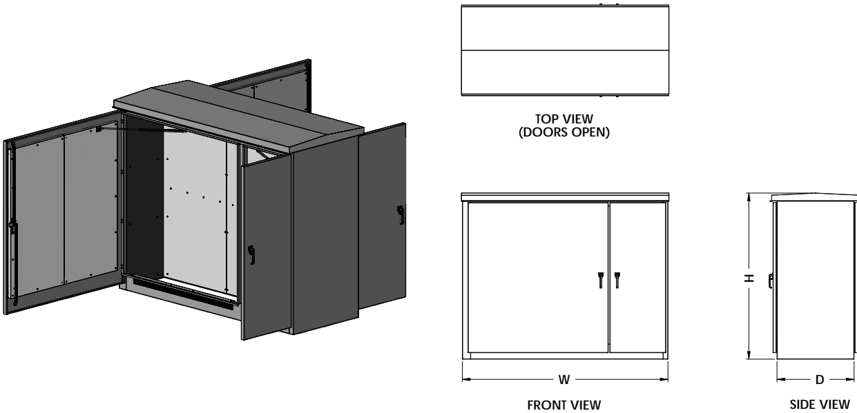
TYPICAL DDS PADMOUNT ENCLOSURE DRAWING
